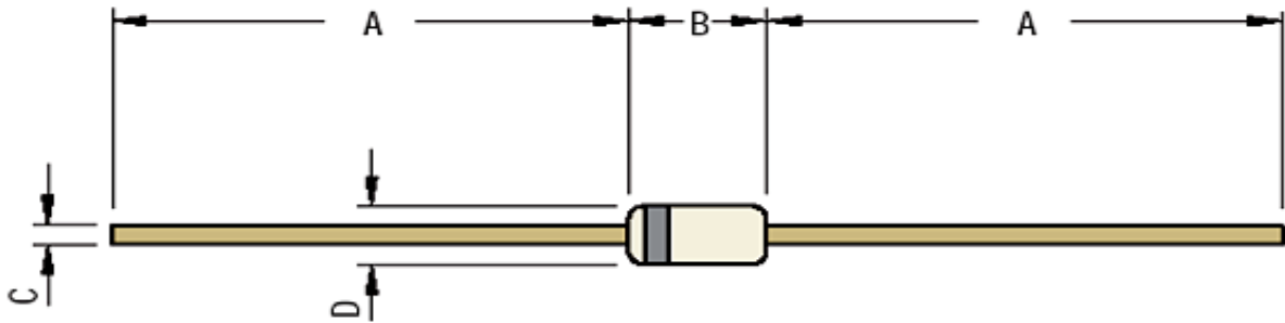
A-405 Axial Leaded Plastic Package
