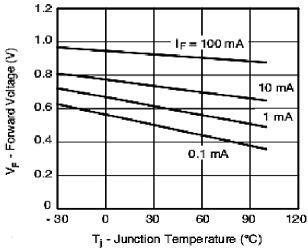
Fig 1: Forward Voltage vs. Junction Temperature
