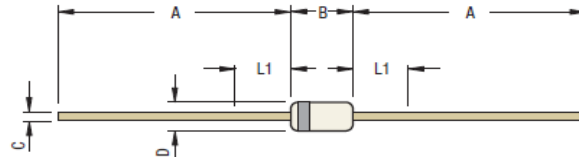
DO-35 Leaded Glass Axial Package
