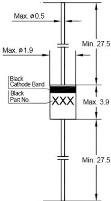
Glass Case DO-35 Dimensions in mm
