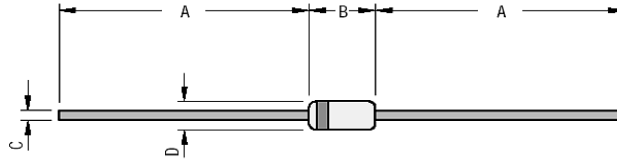
DO-201AD Axial Plastic Package
