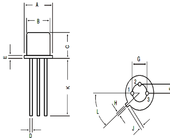
TO-18 Metal Can Package
