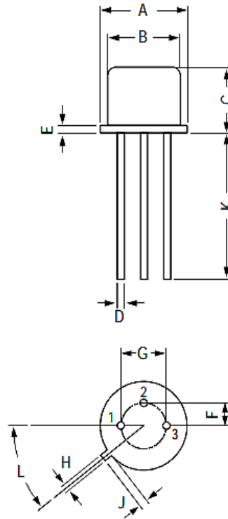
TO-39 Metal Can Package
