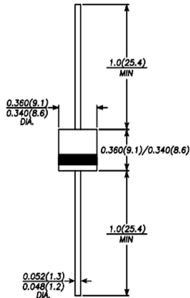
R-6 Leaded Package
