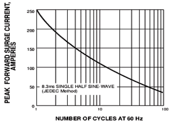
Fig 4: Maximum Non-Repetitive Peak For Forward Surge Current
