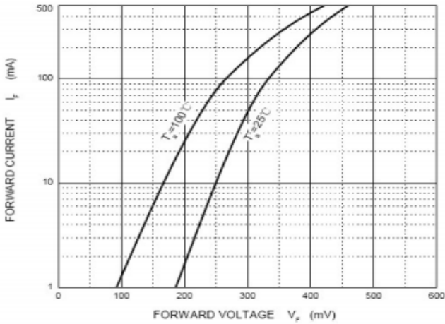
Fig 1: Forward Characteristics
