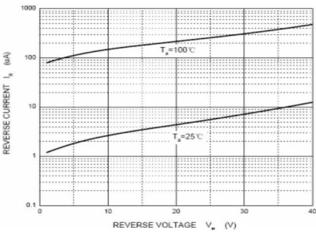
Fig 2: Reverse Characteristics
