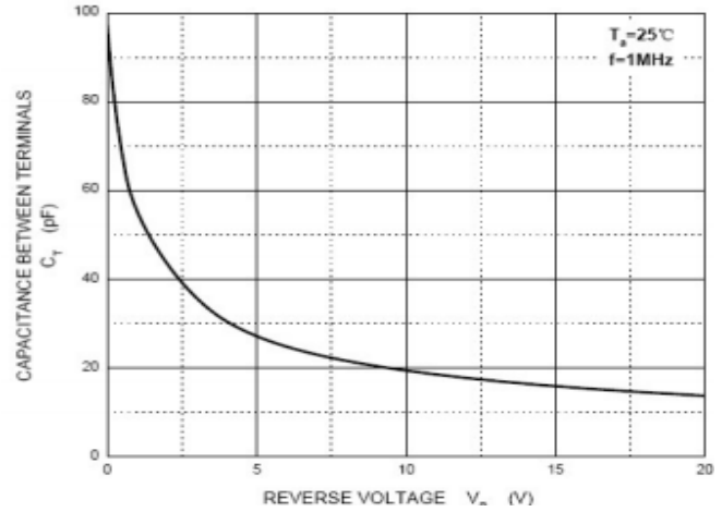
Fig 3: Capacitance Characteristics
