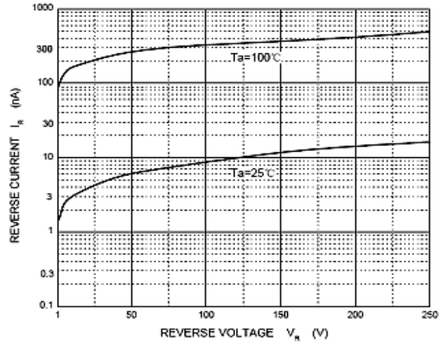
Fig 3: Reverse Characteristics
