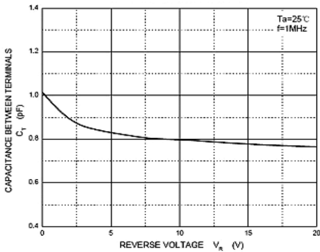
Fig 2: Capacitance Characteristics
