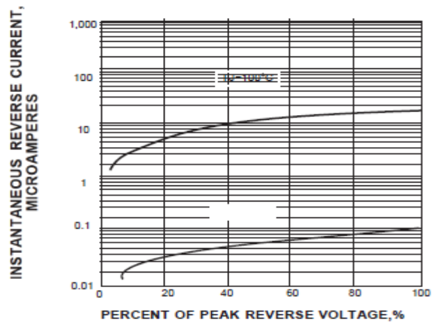
FIG. 4-TYPICAL REVERSE CHARACTERISTICS
