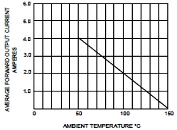
Fig 3: Derating Curve Output Rectified Current
