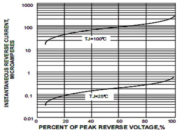
Fig 5: Typical Reverse Leakage Characteristics
