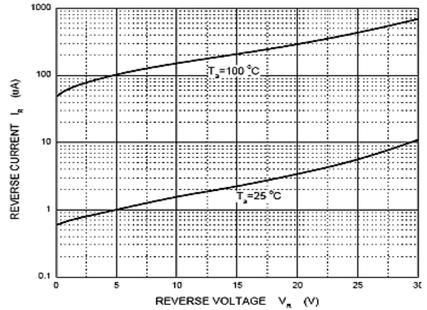
Fig 3: Reverse Characteristics
