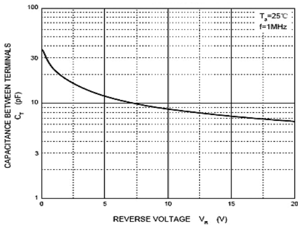
Fig 2: Capacitance Characteristics
