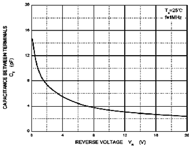
Fig 2: Capacitance Characteristics
