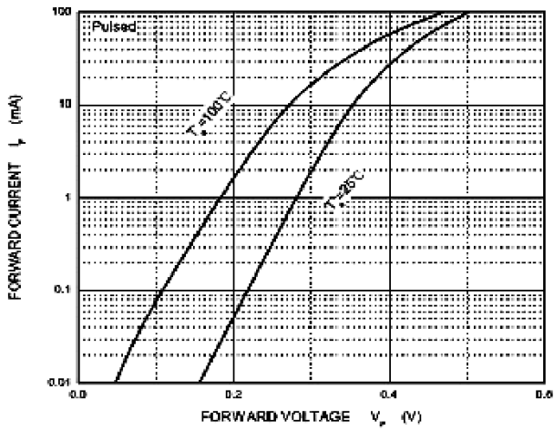
Fig 1: Forward Characteristics
