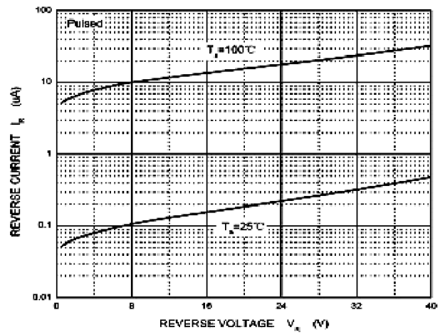
Fig 3: Reverse Characteristics
