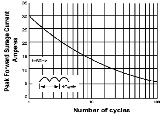
Figure 3. Maximum Non-Repetitive Peak Forward Surge Current per leg
