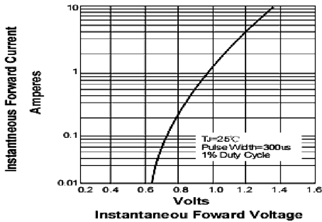
Fig 2: Forward Voltage Characteristics
