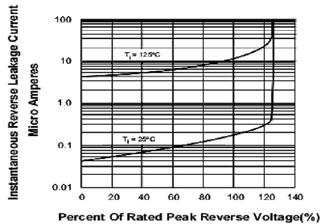
Fig 4: Reverse Leakage Characteristics
