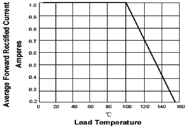
Figure 1. Derating Curve Output Rectified Current
