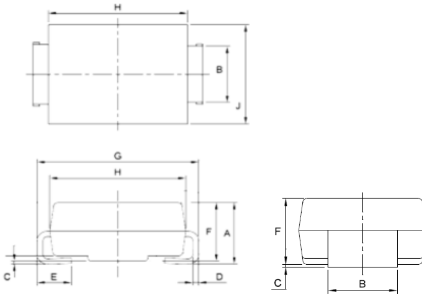
DO-214AA (SMB) Package Outline and Dimension
