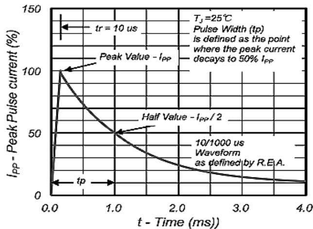
Fig 2: Pulse Waveform
