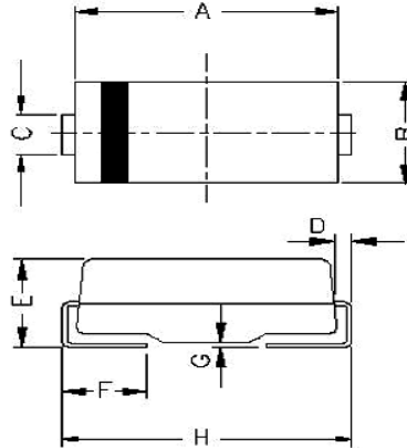
DO-214AA (SMB) Plastic Package
