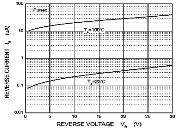
Fig 3: Reverse Characteristics
