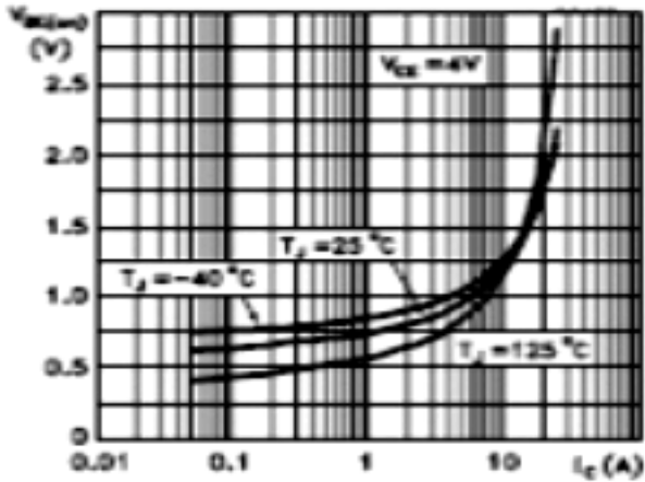
Fig 8: Base Emitter on Voltage for NPN type
