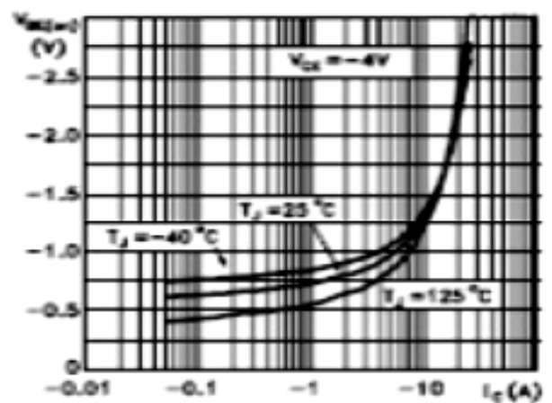
Fig 10: Base Emitter on Voltage for PNP type
