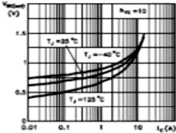
Fig 7: Base Emitter Saturation Voltage for NPN type
