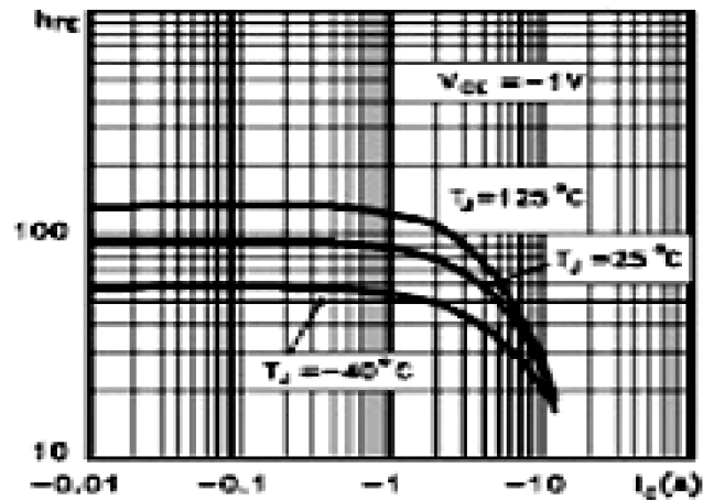
Fig 5: DC Current gain for PNP type
