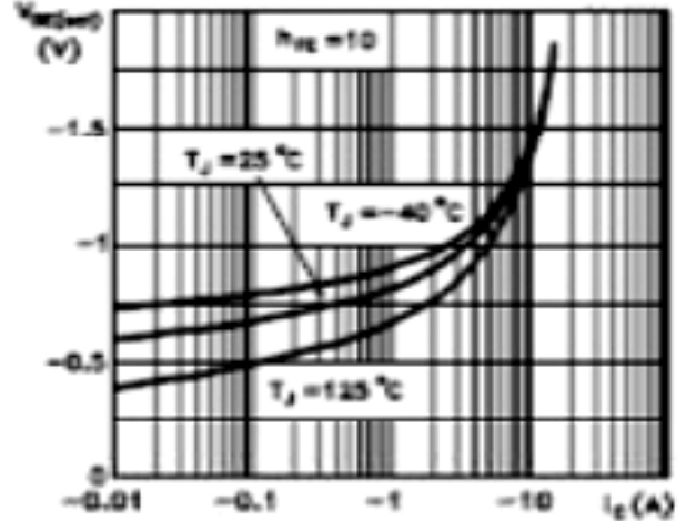
Fig 9: Collector Emitter Saturation Voltage for PNP type
